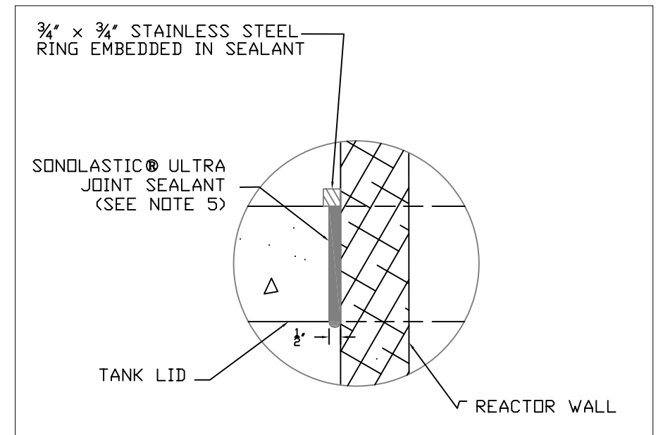
DETAIL A - LID PENETRATION SEAL
