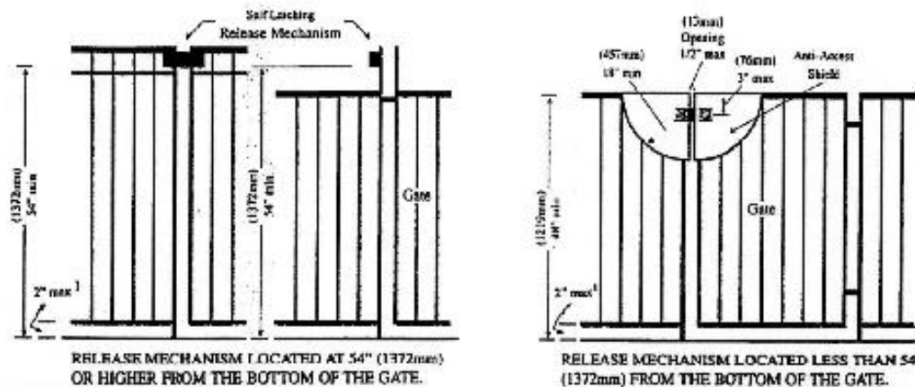
FIG. 4 LATCH RELEASE MECHANISM.
